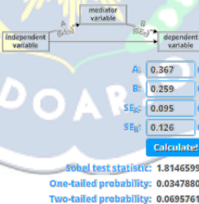
Gambar 3.3 Uji Sobel X3
